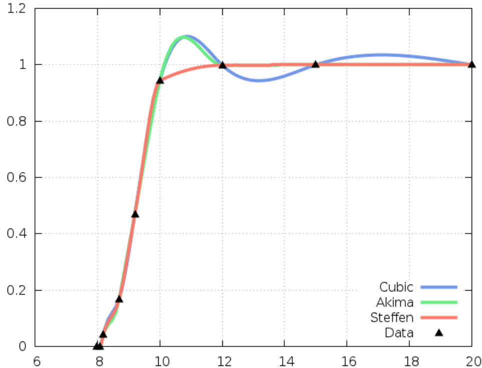
Fig. 30.3: Comparison of different 1D interpolation methods
