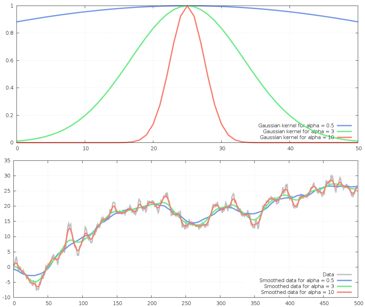
Fig. 24.1: Top panel: Gaussian kernels (unnormalized) for \alpha = 0.5, 3, 10 . Bottom panel: Time series (gray) with Gaussian filter output for same \alpha values.
