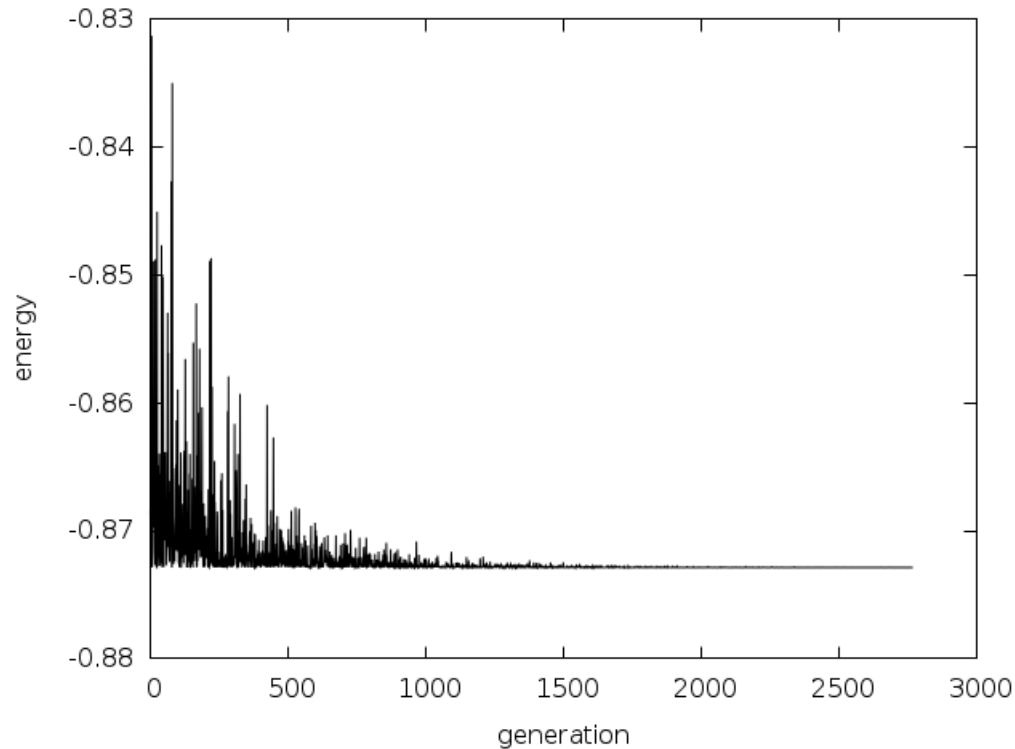
Fig. 28.2: Simulated annealing energy vs generation
