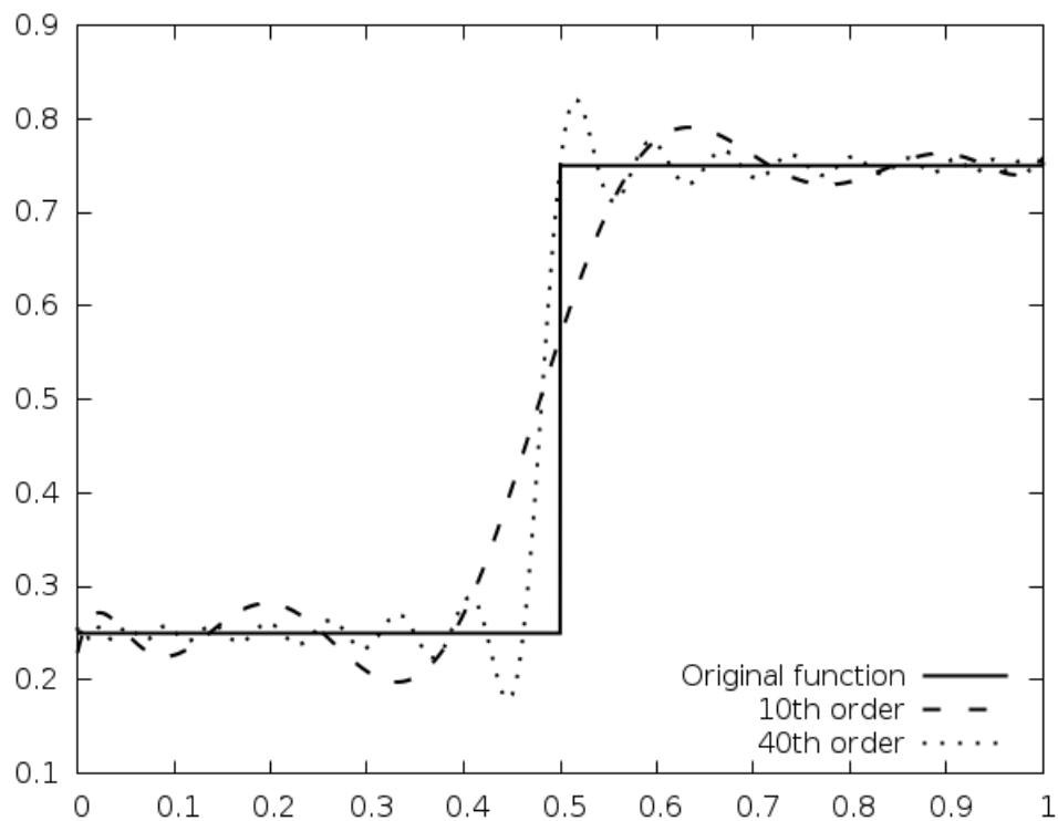
Fig. 32.1: Chebyshev approximations to a step function
